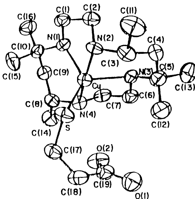
Fig. 9. The structure of [\text{Cu}(\text{tetb})(\text{SCH}_2\text{CH}_2\text{CO}_2)] \cdot 2\text{CH}_3\text{OH} .
