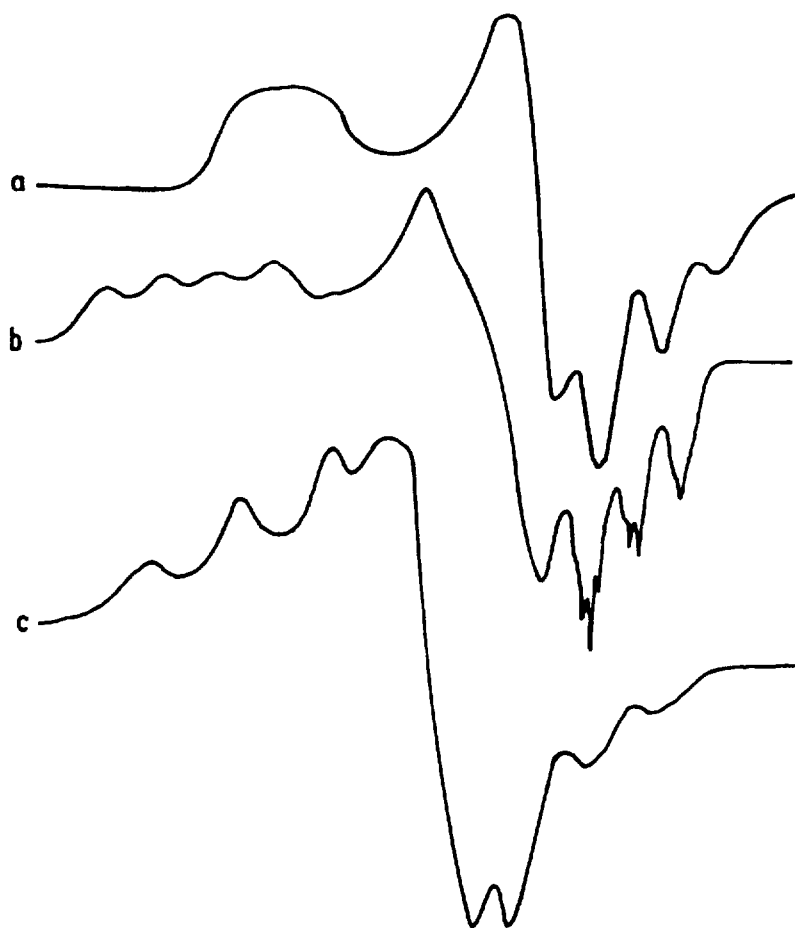
Fig. 29. The X-band EPR spectra of (a) stellacyanin (b) Cu(II)-doped [\text{Zn}(\text{1,2-dimethylimidazole})_2\text{Cl}_2] and (c) \text{CuN}_2\text{S}_2 complex (in MeCN glass) of the aliphatic ligand shown in Fig. 19.
